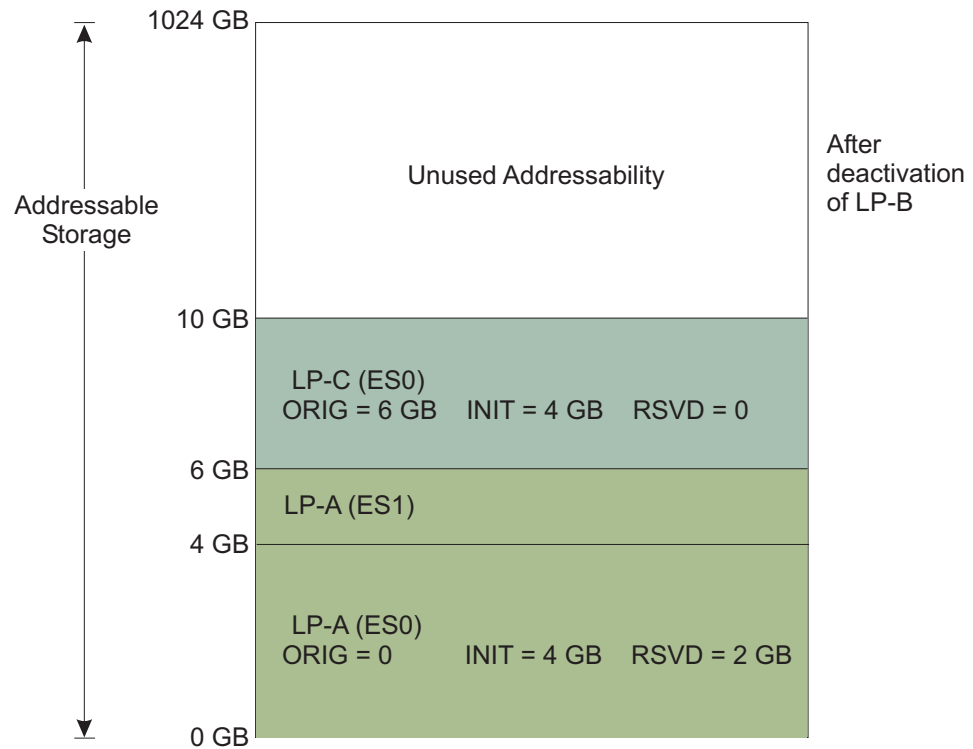
Figure 3-8. Reconfigured Expanded Storage Layout
