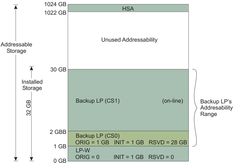
Figure 3-15. Backup Partition Layout After Nonspecific Deactivation
