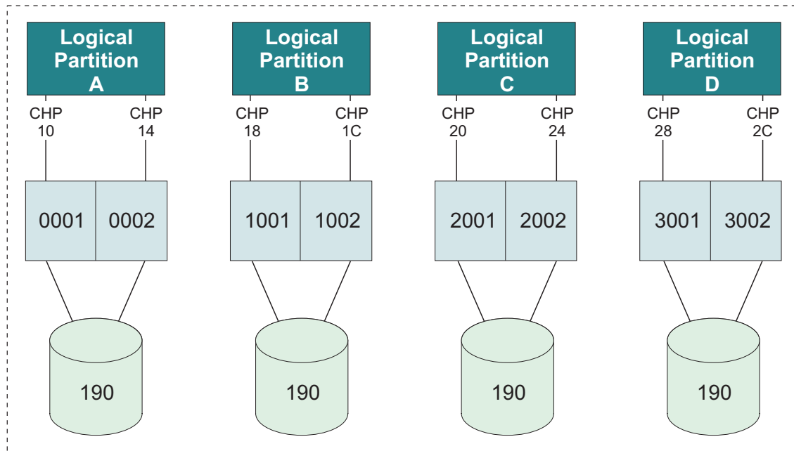
Figure 2-14. Logical View of Shared Device 190
