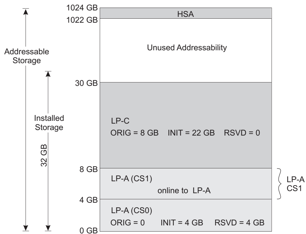
Figure 3-2. Reconfigured Central Storage Layout
