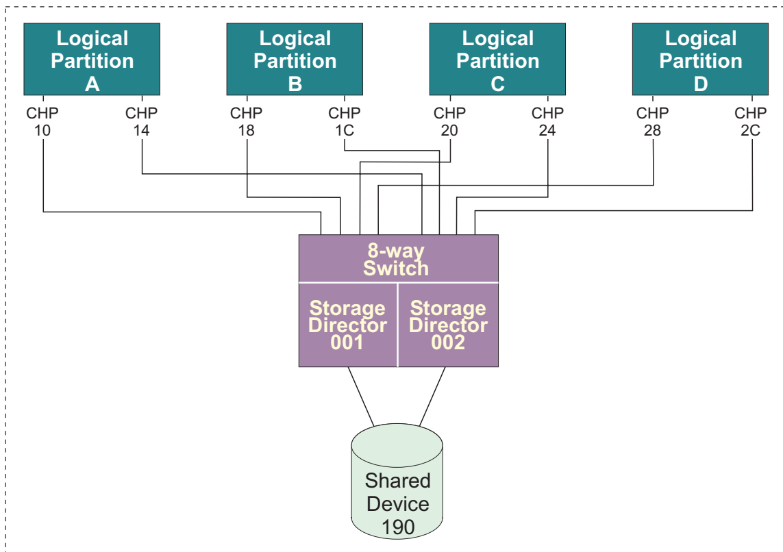
Figure 2-13. Physical Connectivity of Shared Device 190
