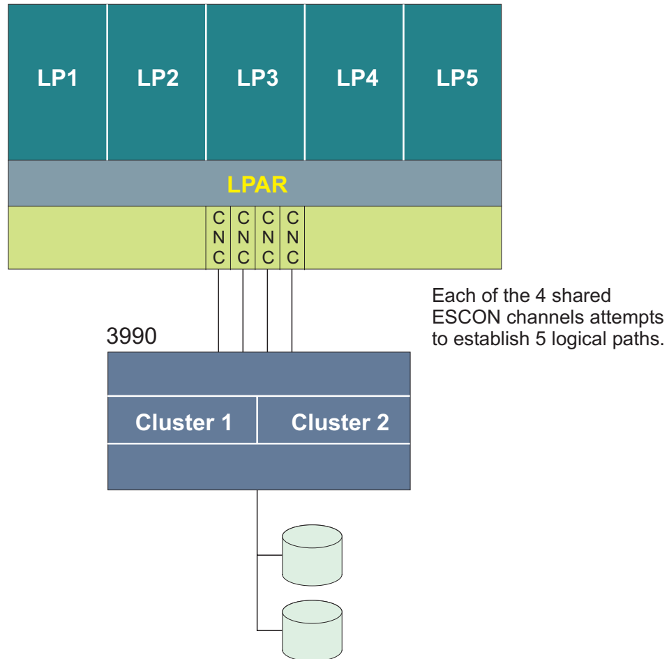
Figure 2-2. A Shared ESCON Configuration that Can Benefit from Better Logical Path Management
