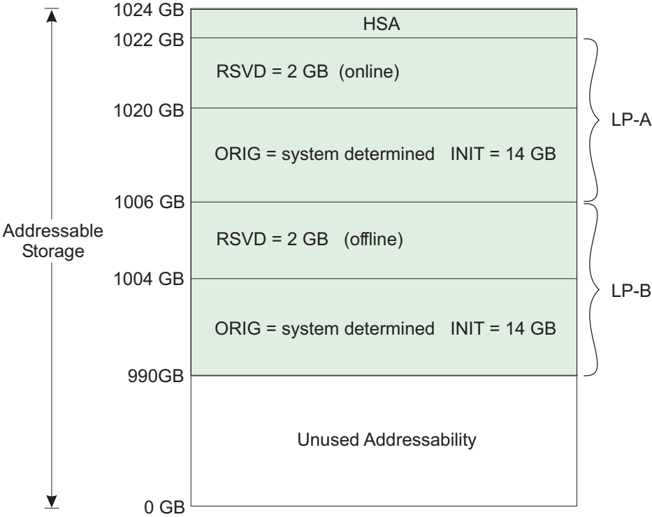
Figure 3-3. Initial Central Storage Layout
