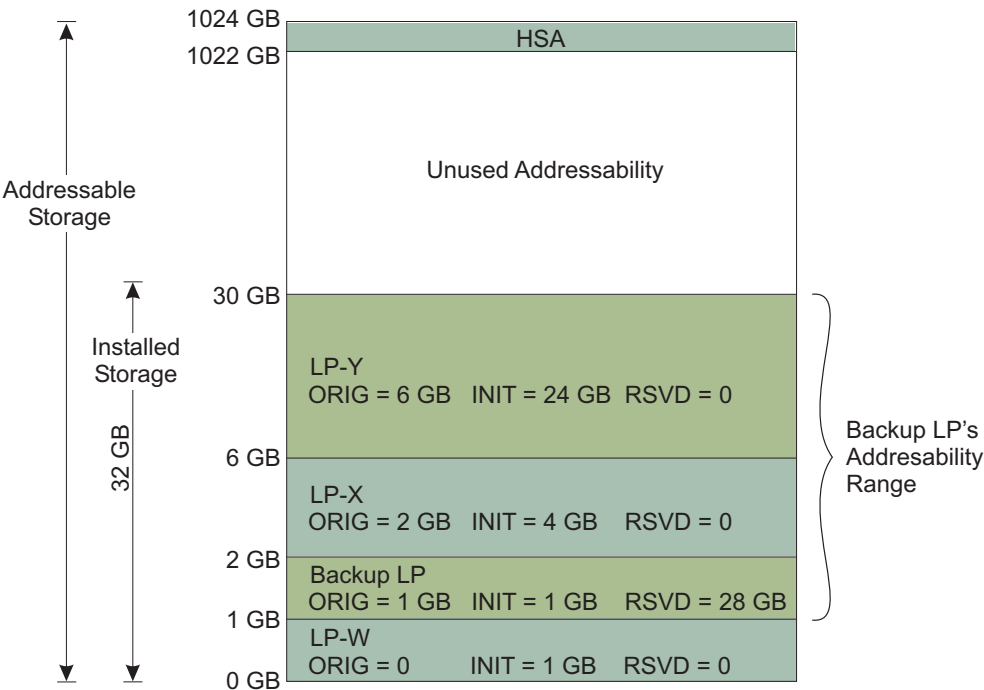
Figure 3-14. Backup Partition Layout Before Nonspecific Deactivation
