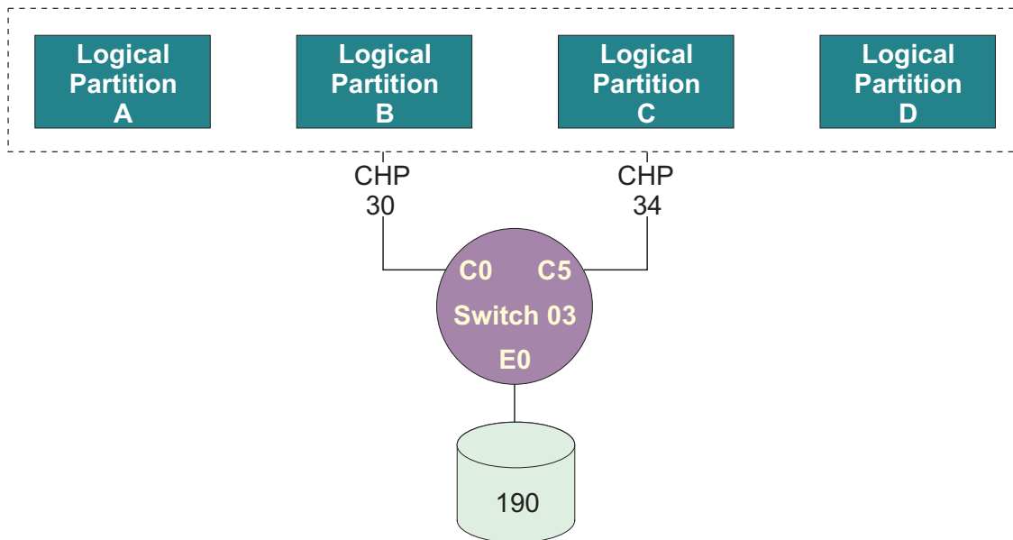
Figure 2-12. Shared Devices Using Shared ESCON Channels
