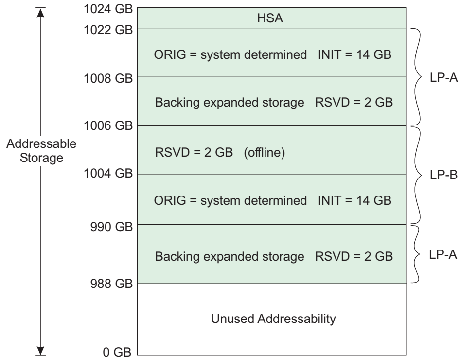
Figure 3-12. Central Storage Layout Following Reconfiguration
