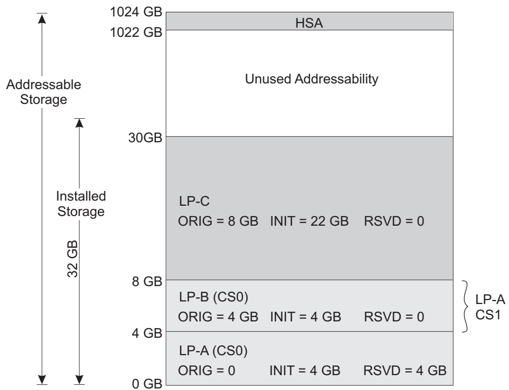
Figure 3-1. Central Storage Layout
