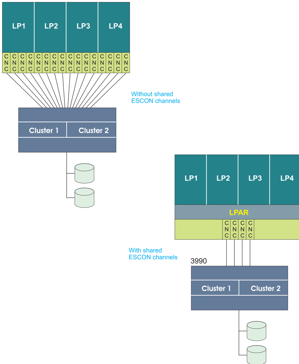
Figure 2-9. Consolidating ESCON Channels and ESCON Control Unit Ports
