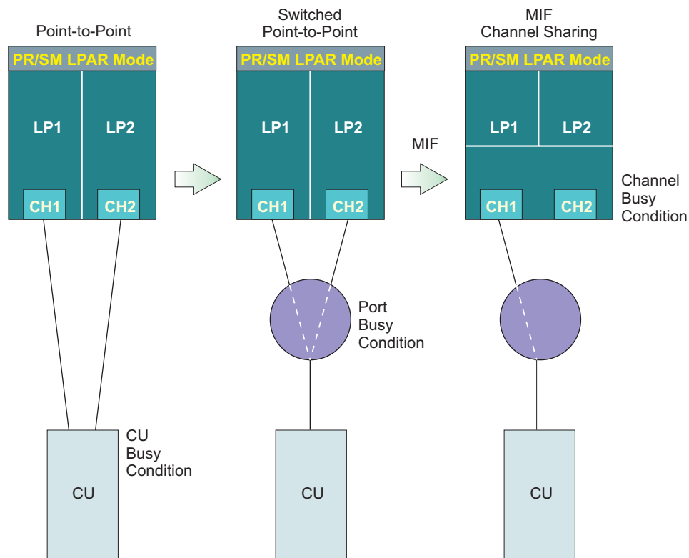
Figure 2-8. Progression of Busy Condition Management Improvements
