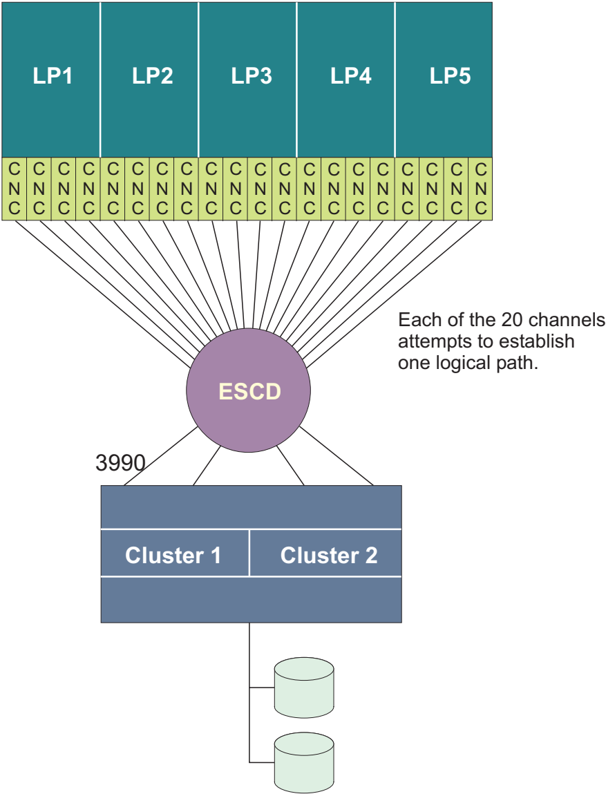
Figure 2-1. An ESCON Configuration that Can Benefit from Better Logical Path Management
