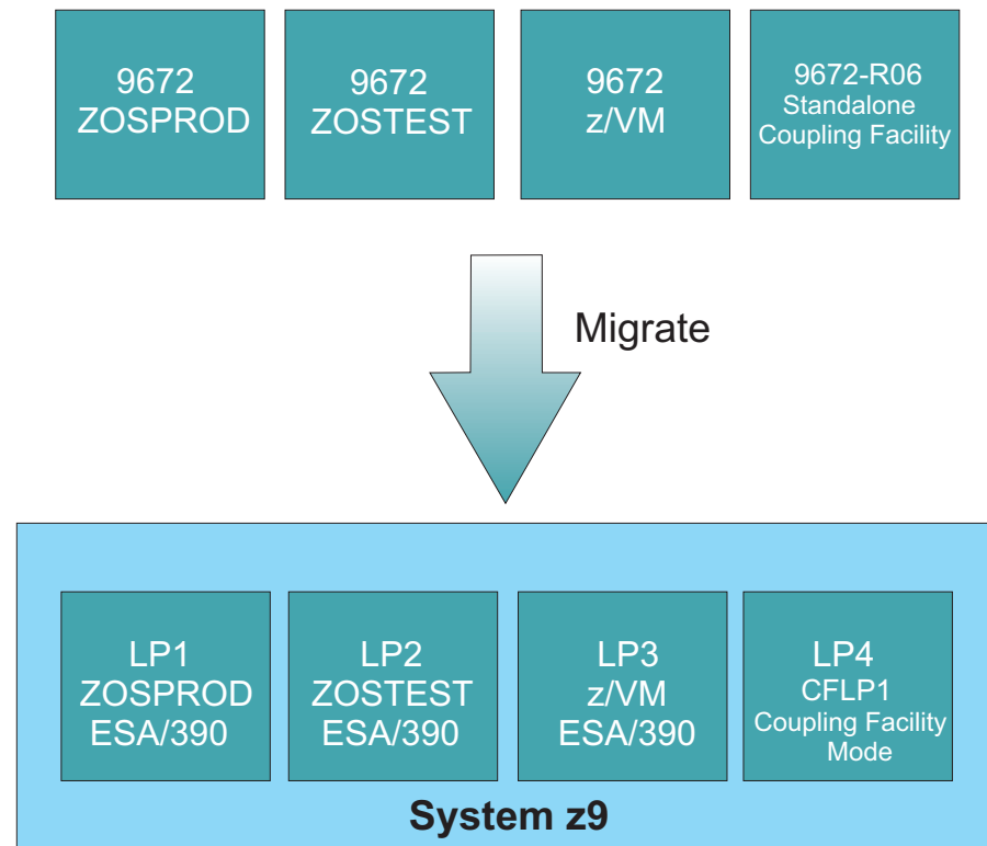
Figure 1-2. Migration of Four Production Systems to LPs
