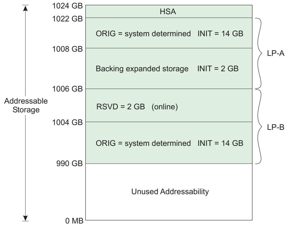
Figure 3-10. Initial Central Storage Layout
