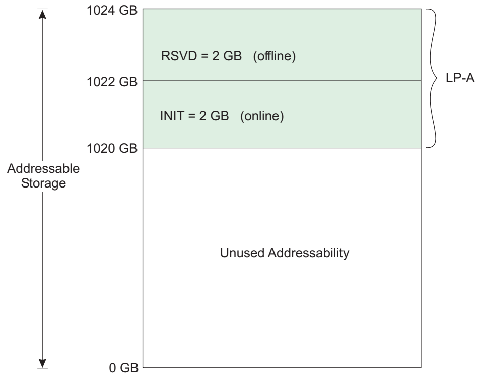
Figure 3-11. Initial Expanded Storage layout
