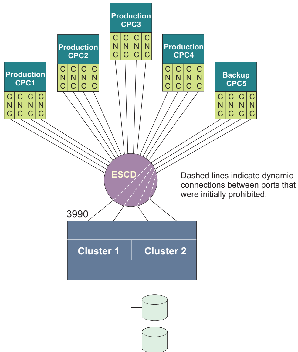
Figure 2-7. Using the ESCD to Manage Logical Paths by Prohibiting Dynamic Connections
