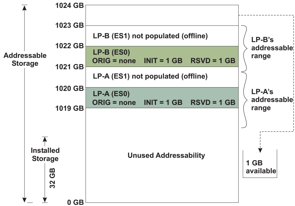
Figure 3-9. Expanded Storage Layout
