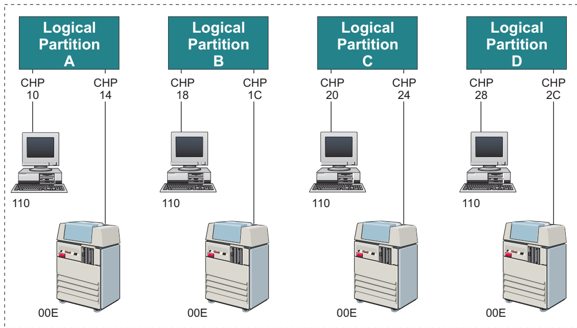
Figure 2-15. LPAR Configuration with Duplicate Device Numbers
