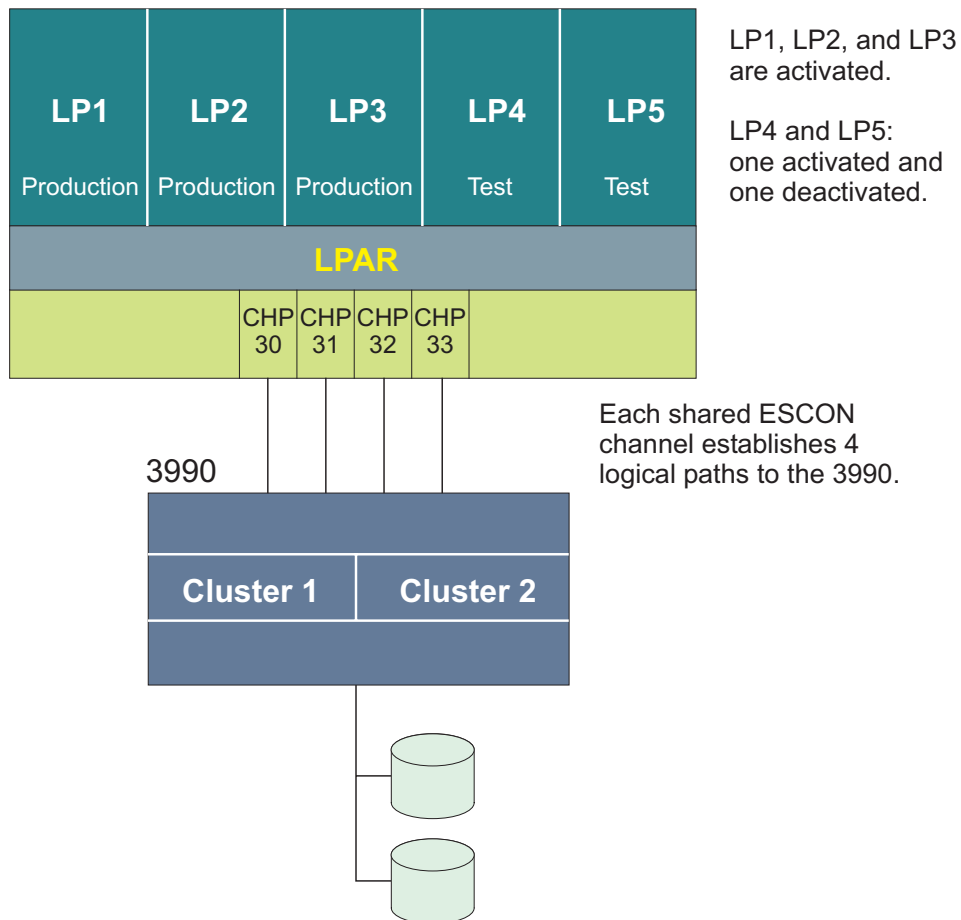
Figure 2-3. Deactivating Unneeded Logical Partitions
