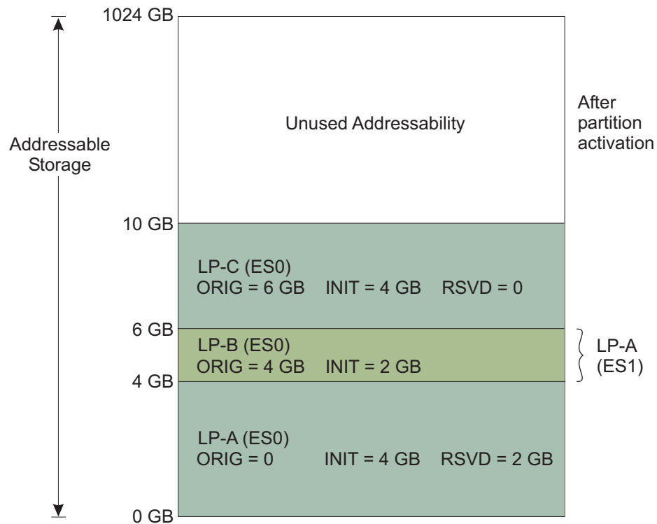
Figure 3-7. Expanded Storage Layout
